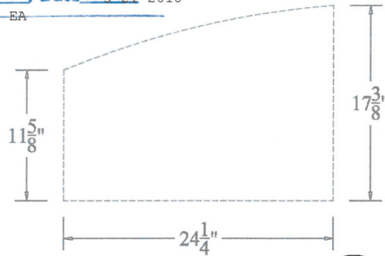
Glass Panel
