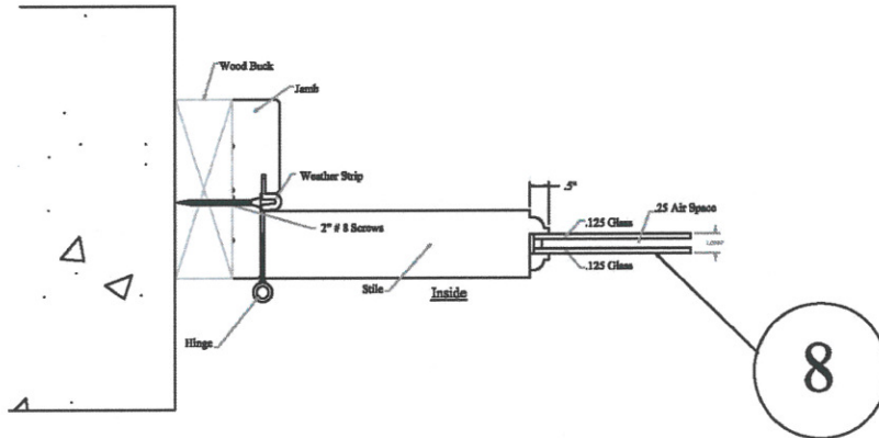
Ⓒ Anchor Section
