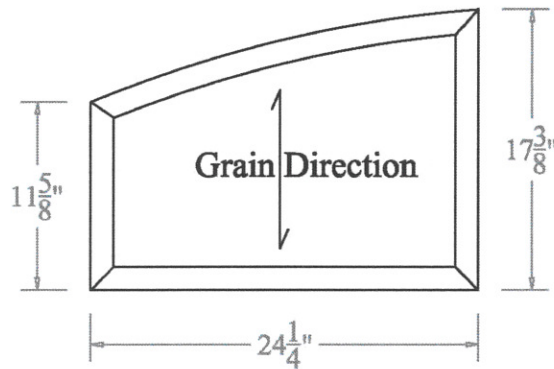
Wood Panel
