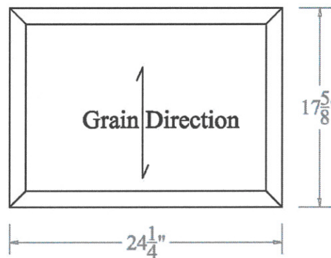
Wood Panel
